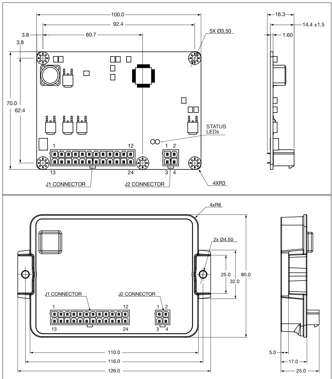
Figure 2-1 Mounting dimensions, Curtis 1356 and 1356P expansion modules.
