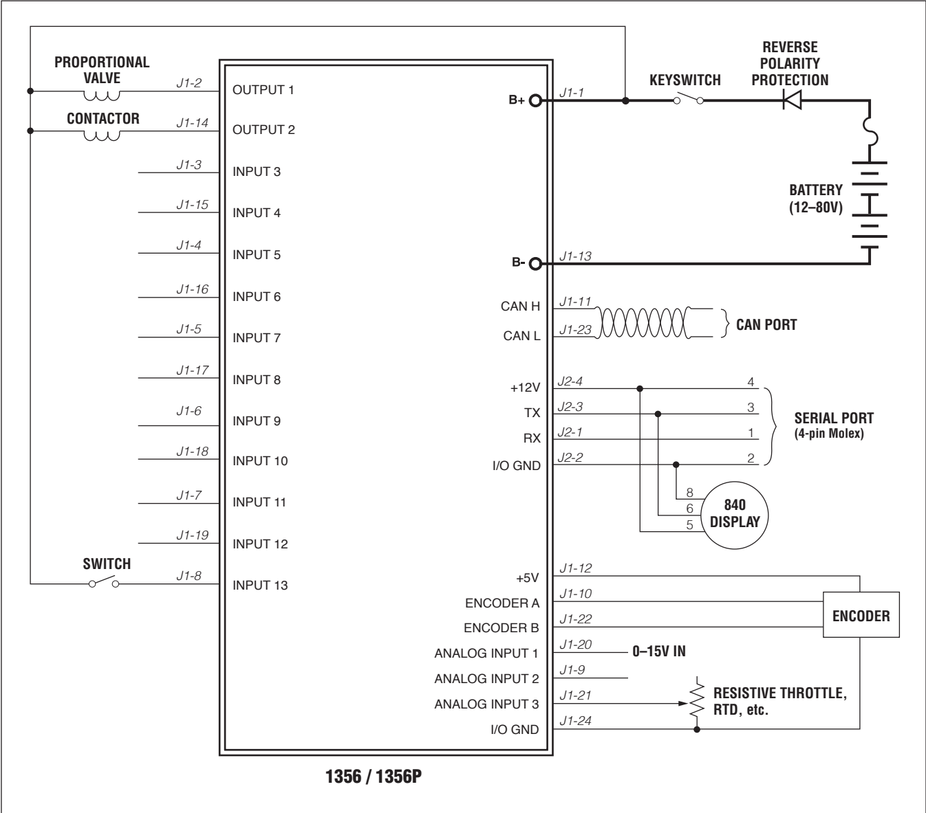
Figure 2-2 Basic wiring diagram, Curtis 1356 /1356P CAN expansion module.
